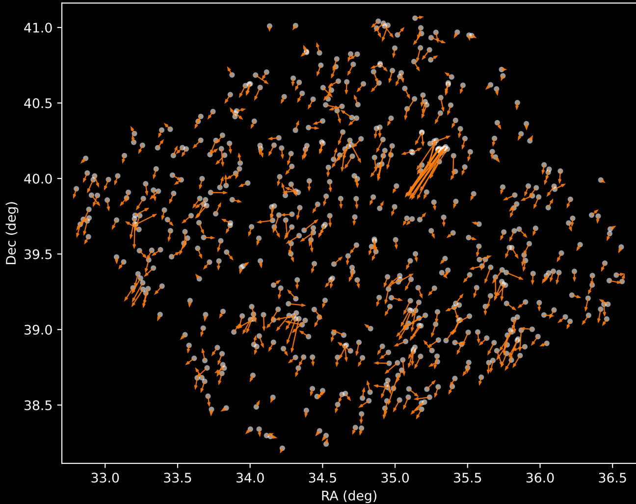
APOGEE DR17 Cluster 2 Proper Motion Vectors (n=585)
