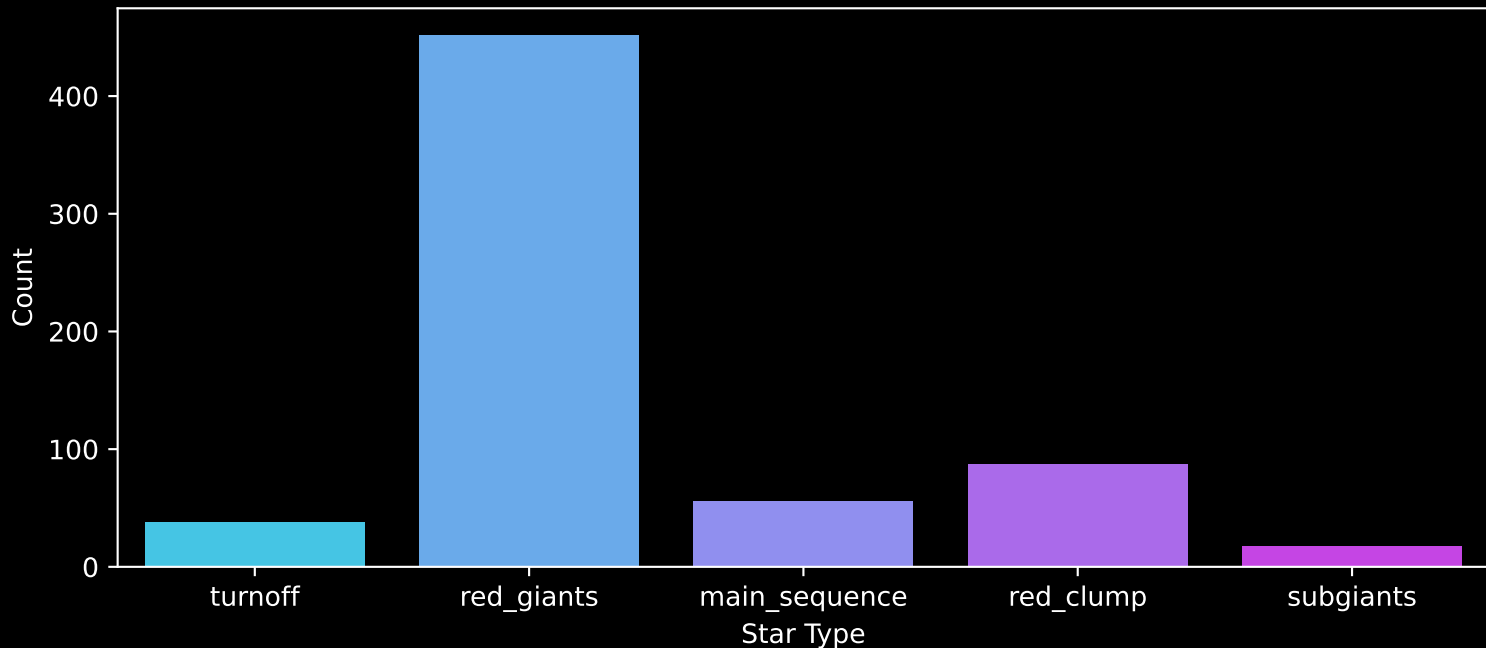
APOGEE DR17 Field: [K20_073+09] Count plot of Star Type
