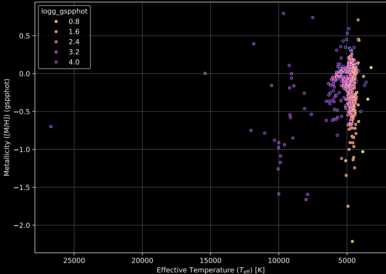
APOGEE DR17 Field: [K20_073+09] Stellar Population Parameters (n= 650)
