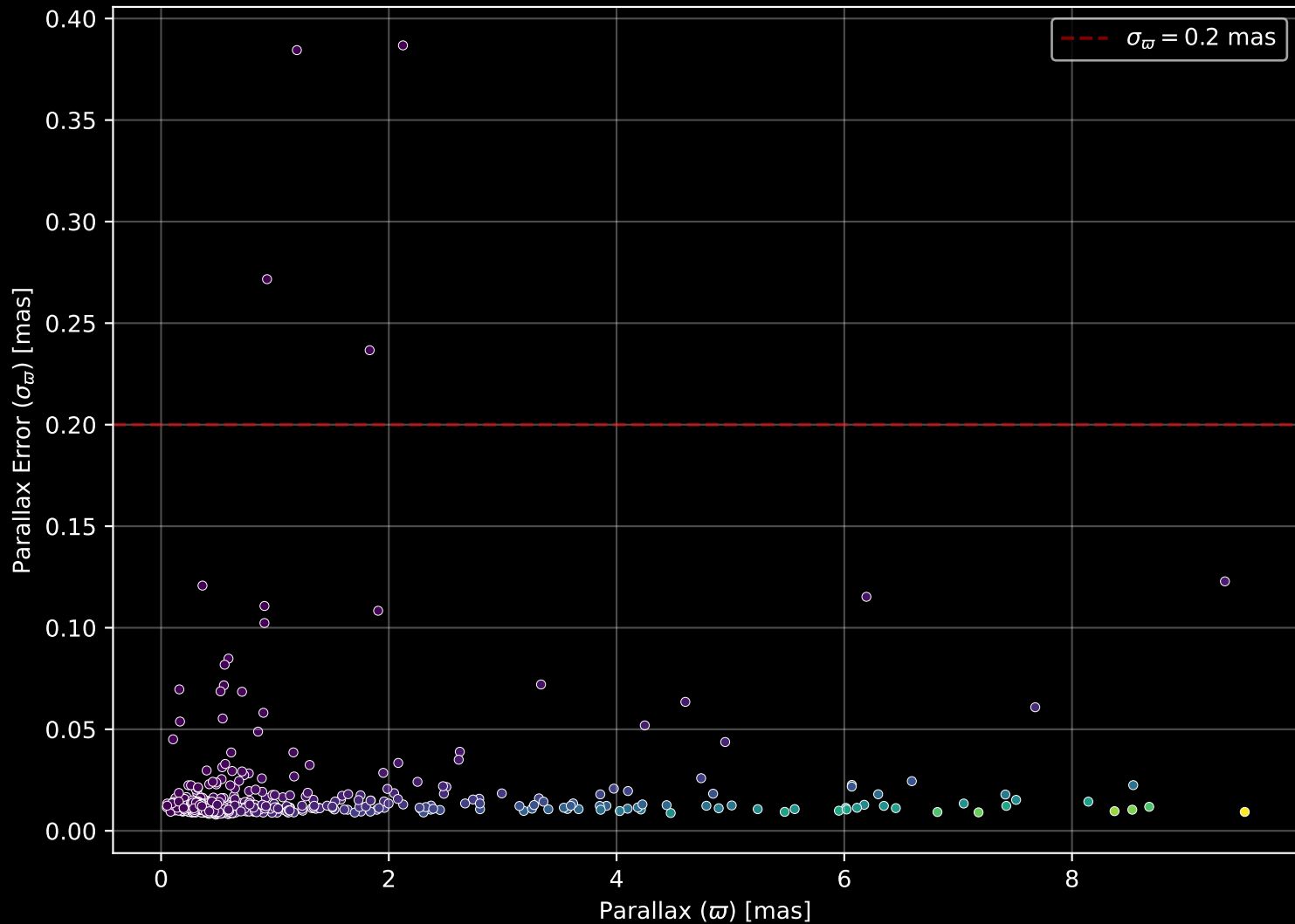
APOGEE DR17 Field: [K20_073+09] Parallax Quality (n= 650)
