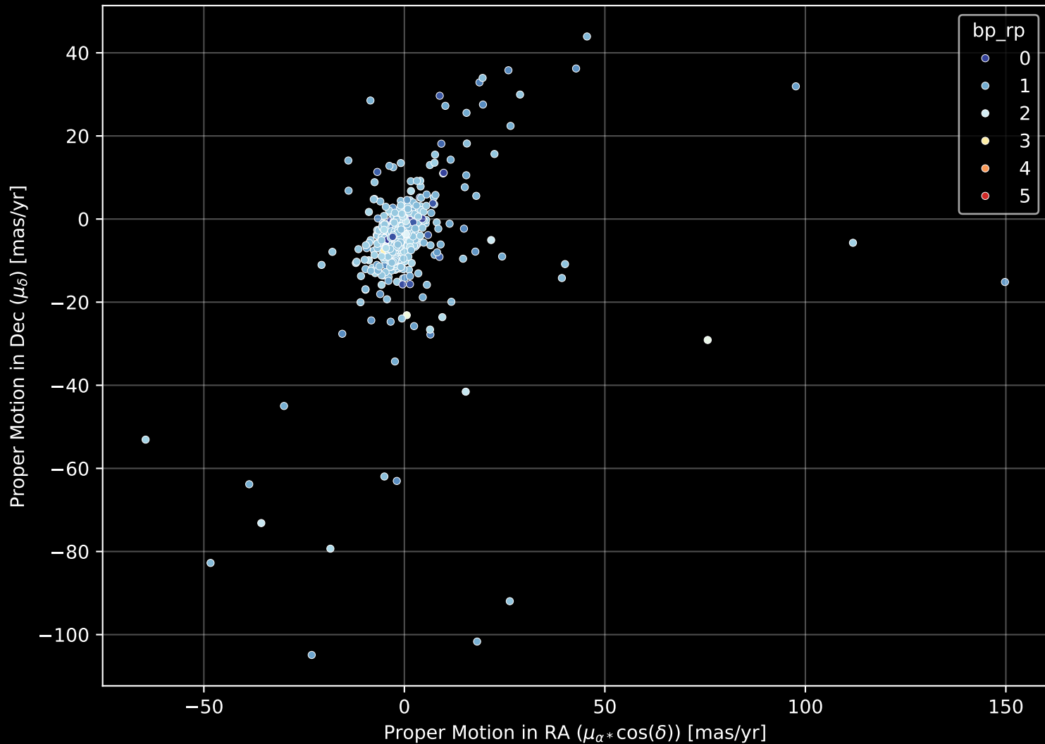
APOGEE DR17 Field: [K20_073+09] Proper Motion Diagram (n= 650)
