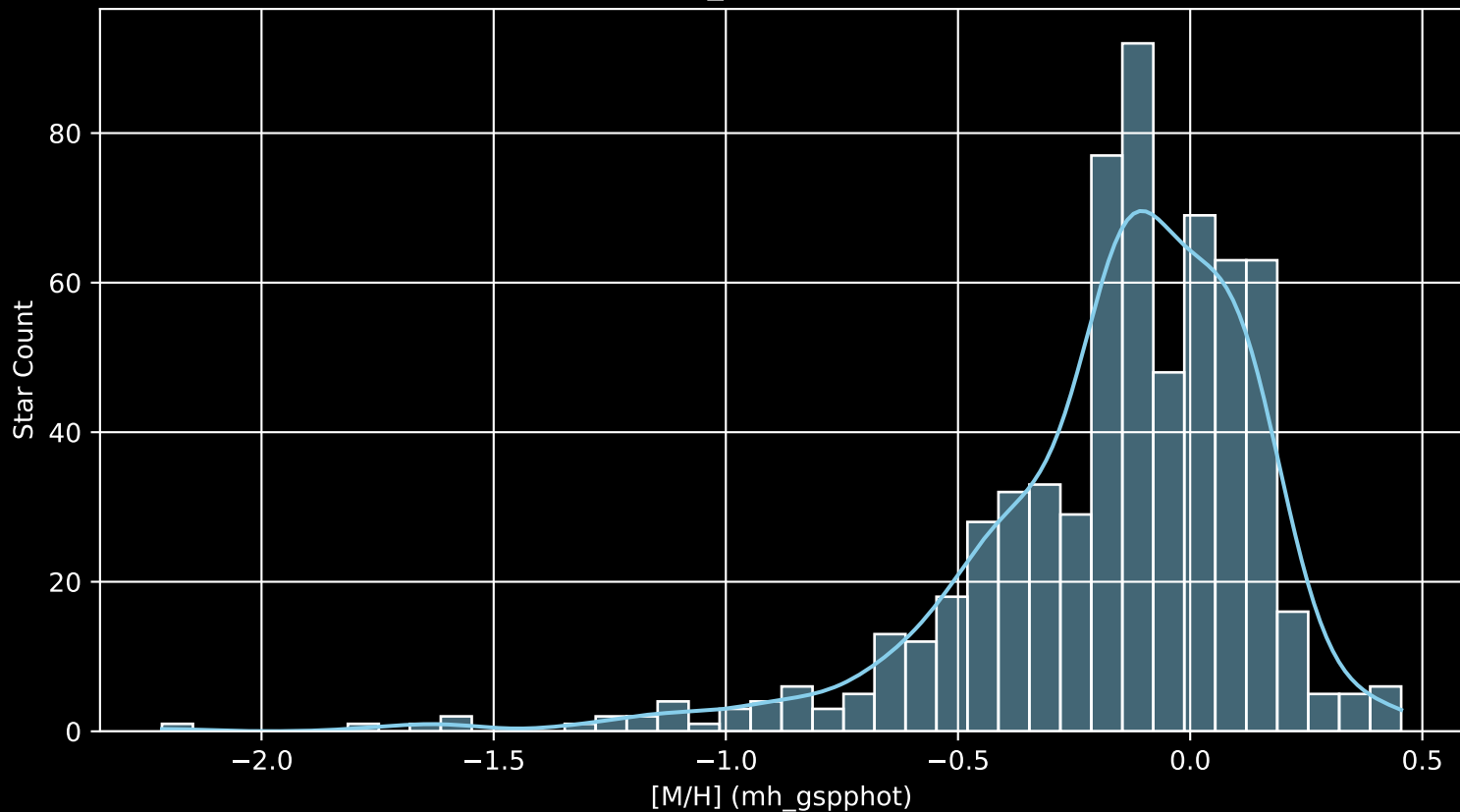
APOGEE DR17 Field: [K20_073+09] [M/H] (mh_gspphot) (n= 645)
