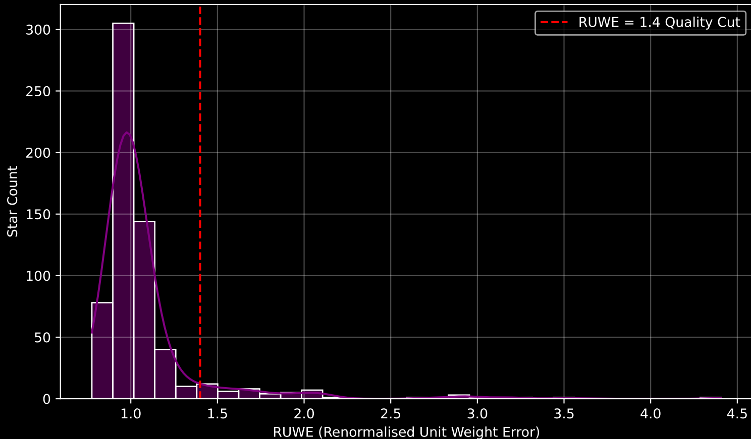
GAPOGEE DR17 Field [K20_073+09] RUWE Distribution (n= 629)
